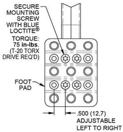
FOOT PAD DETAIL
